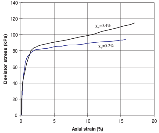
Figure 18. Stress-strain behavior of specimens prepared using \chi_w = 0.2, 0.4\% , with l_f = 25 mm fibers (2610 denier), \sigma_3 = 116 kPa, Soil 2.
