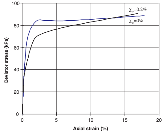
Figure 16. Stress-strain behavior of specimens prepared using \chi_w = 0, 0.2\% , with l_f = 50 mm fibers (2610 denier), \sigma_3 = 98 kPa, Soil 2.
