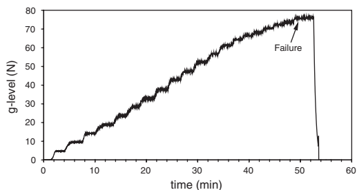
Figure 4. G-level (N) versus time during centrifuge testing.
