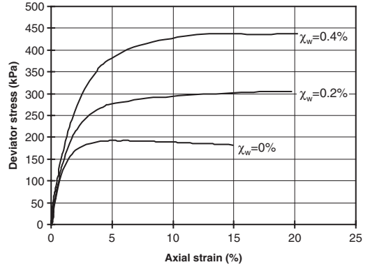
Figure 12. Stress-strain behavior of specimens prepared using \chi_w = 0, 0.2 and 0.4\% with l_f = 25 mm fibers (360 denier), \sigma_3 = 70 kPa, Soil 1.
