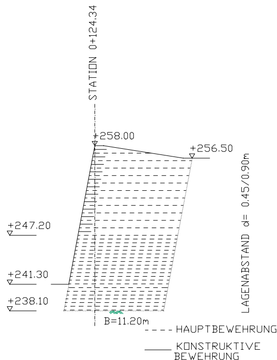
Figure 2: Cross section at chainage 0+124,34
