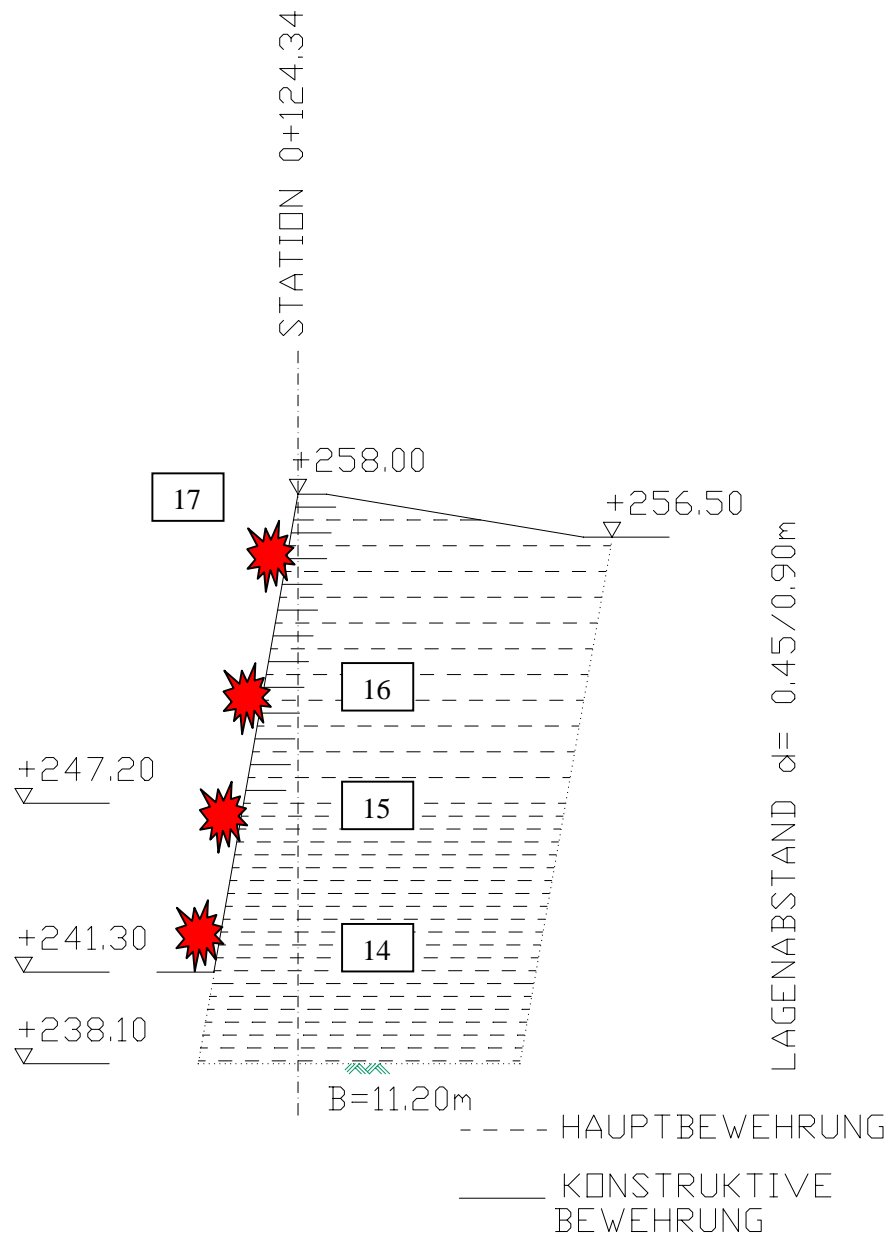
Figure 12: Cross section with measurement points
