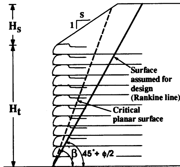
Fig. 1 Reinforced soil wall with sloping backfill showing potential failure surface assumed in conventional design.
