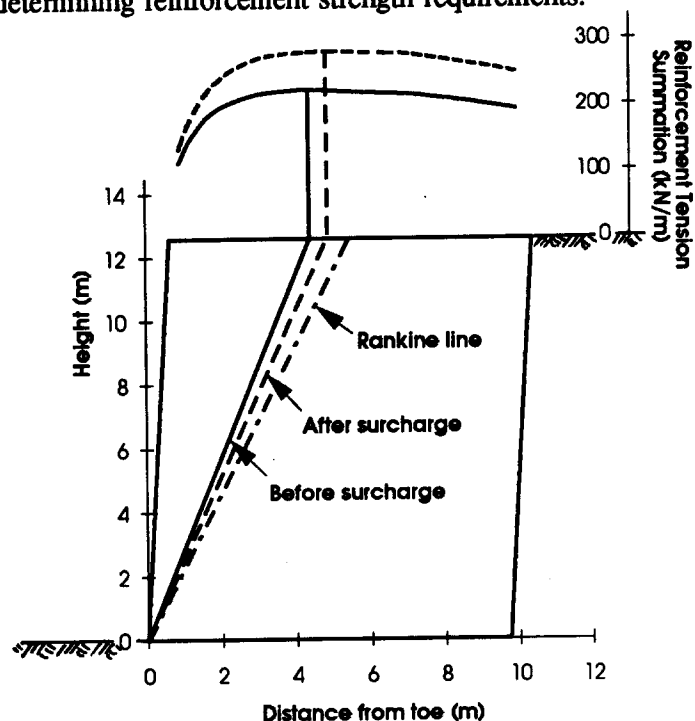
Fig. 3 Location of the planar surfaces with maximum RTS at the Rainier Ave. wall.
