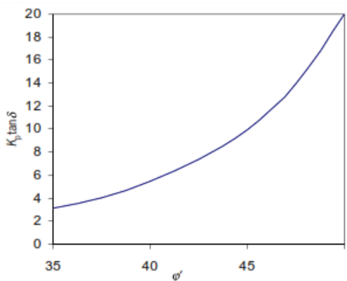
Fig. 2 Design values of K_p \tan \delta (BRE 2004)
