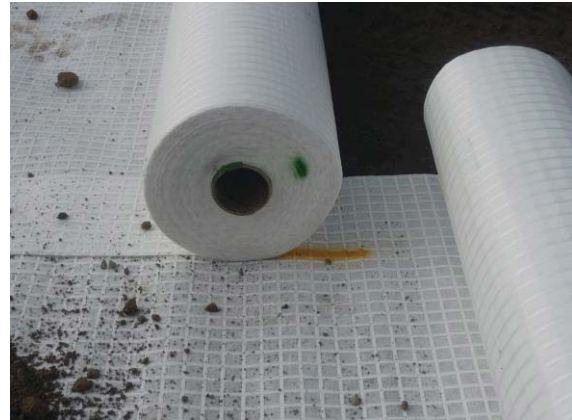
Fig. 5 Installation and overlaps
