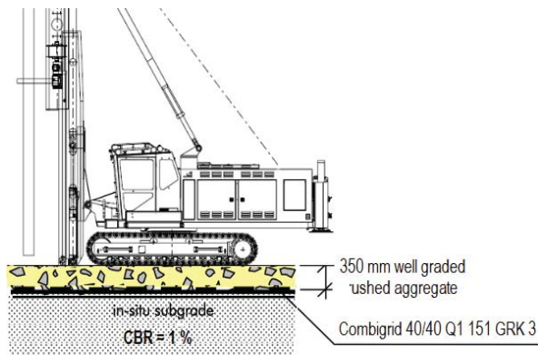
Fig. 3 Reinforced working platform
