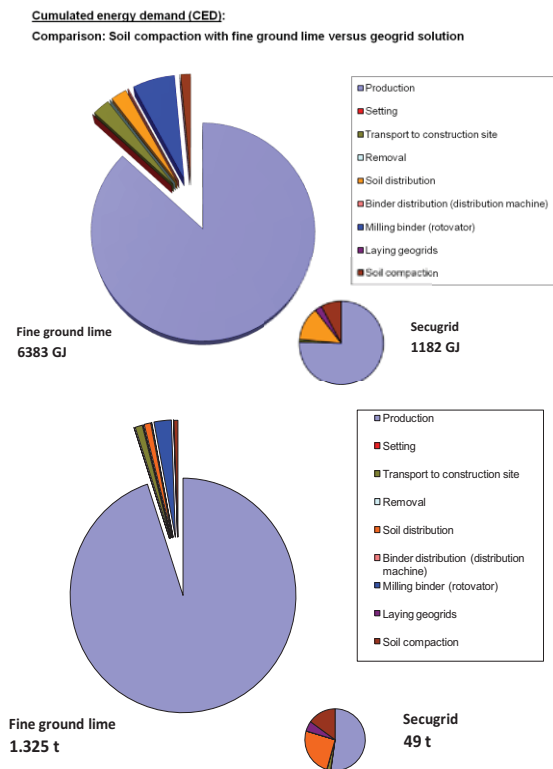
Fig. 9 Cumulated energy demand (CED) and CO 2 emissions at district road K34, district Aix-la-Chapelle, Germany, 2008
