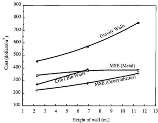
Fig. 3 The money challenge (MSE = Mechanically Stabilized Earth)
