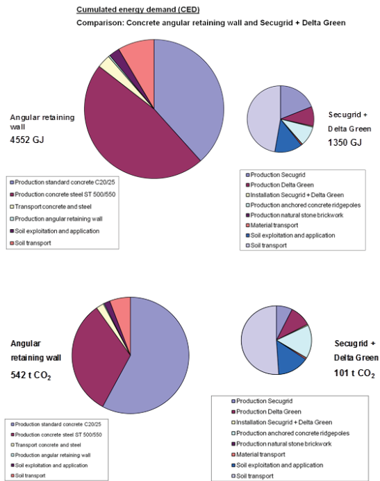
Fig. 6 Cumulated energy demand (CED) and CO 2 emissions at Gänsbergspange near Frankfurt, Germany
