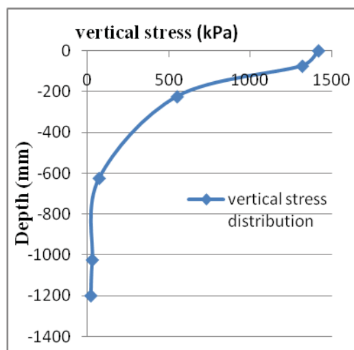
Fig. 9 Pressure distribution below the footing in geocell reinforced case
