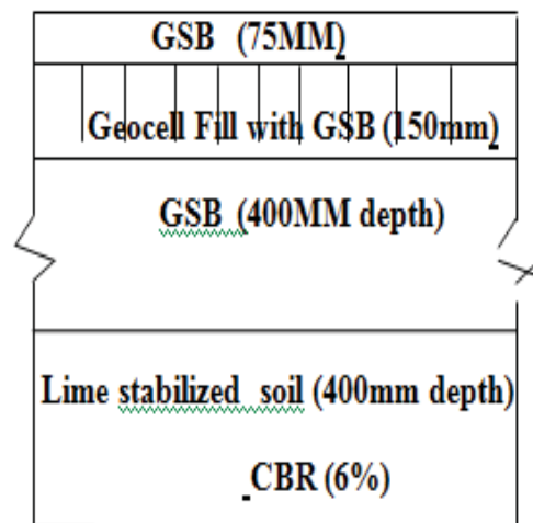
Fig. 1 Cross section of the pavement section at Govind Dairy Factory
