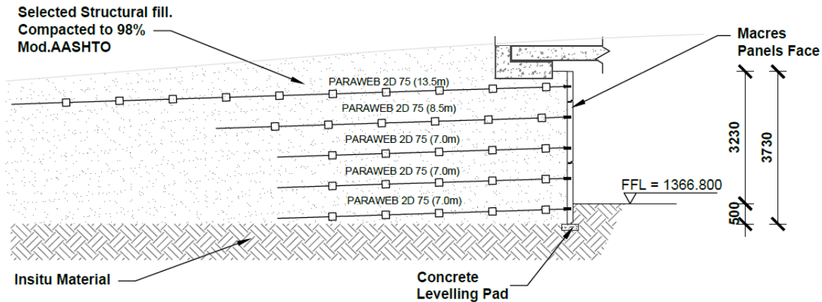
Figure 8. Typical section
