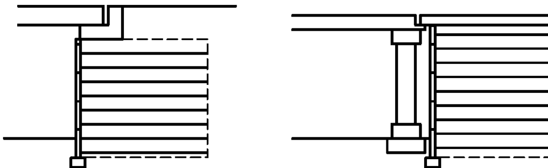
Figure 2. RIGHT: False abutment – LEFT True abutment (BS 8006,2010)
