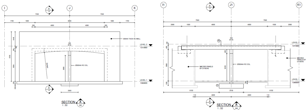
Figure 4 (LEFT). First proposal with false bridge abutment – typical section
