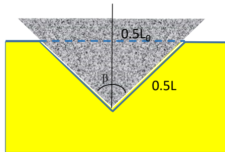
Figure 1. Elongation geotextile due to impact from L_0 to L .
