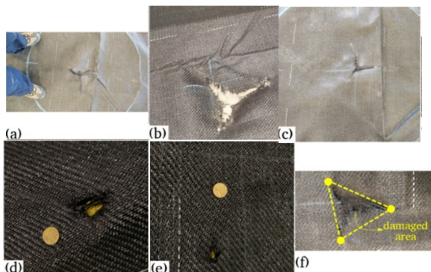
Figure 5. Examples of damaged zones after tests: block B and drop height of 3.0 m (a); block B and drop height of 2.0 m (b); block B and drop height of 1.55 m (c); block A and drop height of 4.0 m (d); block A and drop height of 3.5 m (e); calculation of ruptured area (f). (adapted from Izadi et al., 2017)
