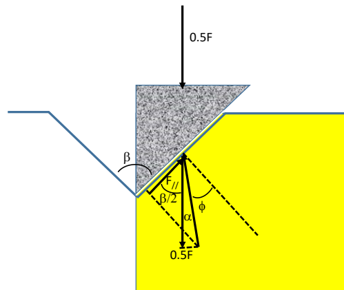
Figure 8. Forces on block and geotextile during impact.
