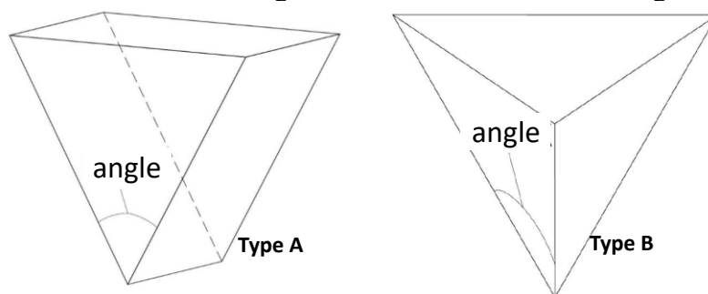
Figure 7. Definition of the angle \beta for Type A and Type B blocks. (De Strijcker and Decraene, 2017)
