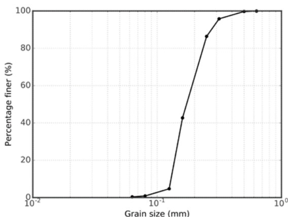
Figure 2. Grain size distribution of the sand
