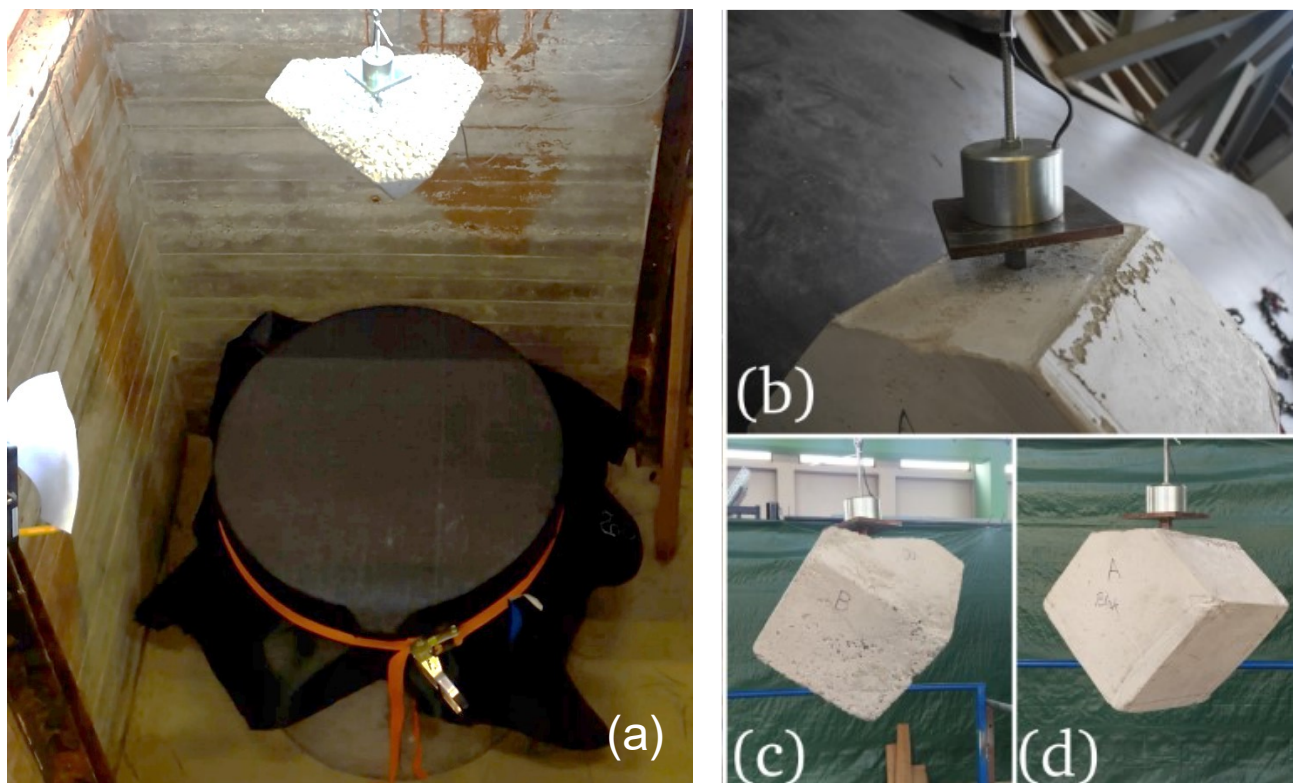
Figure 4. Setup of the experiments (a) and details (b, c and d) (adapted from Izadi et al., 2017)
