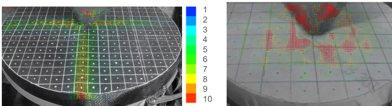
Figure 6. Deformation pattern for woven (left) and non-woven (right) geotextile during impact of a sharp stone (B60). The different colours show the amount of pixels the geotextile has moved. The pictures are originally 1920x1080 pixels (adapted from De Strijcker and Decraene, 2017).
