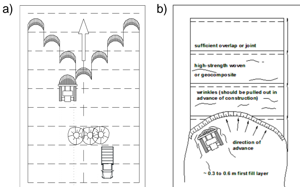
Figure 3. Examples of installation methods of geosynthetics in tailings ponds.
