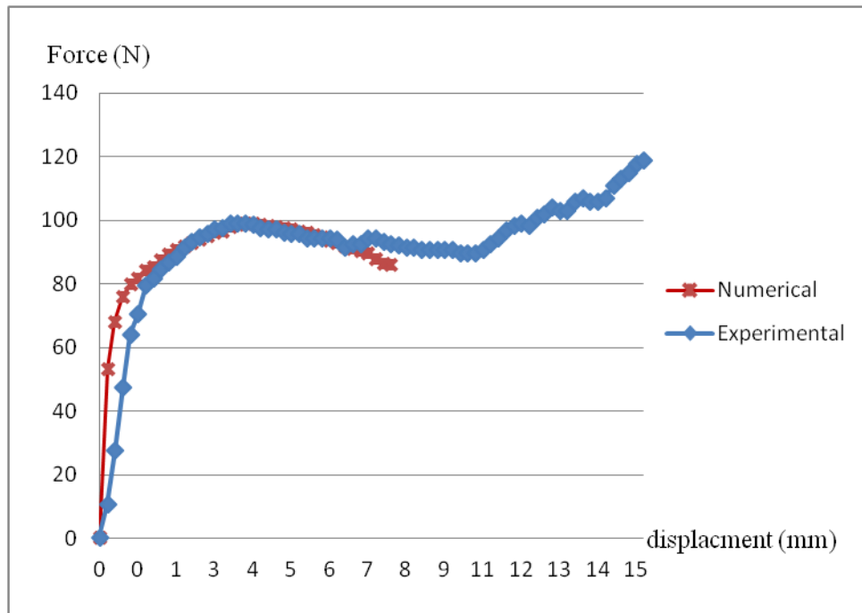
Fig. 5 Force- displacement diagram
