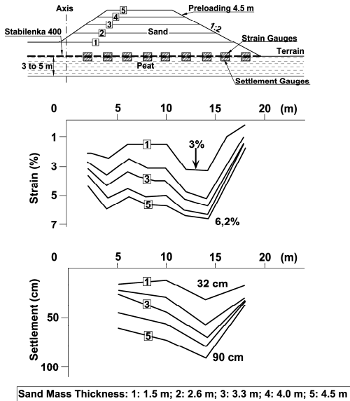
Figure 3. Grossemeer "test section" (TS): construction stages, settlements and strains during the first 4 days in 1986
