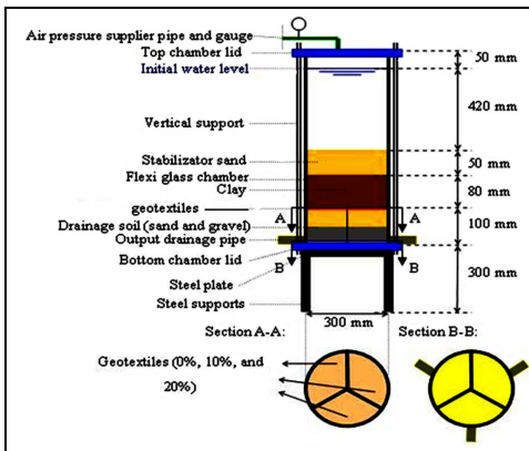
Figure 1. Schematic diagram of clogging test apparatus
