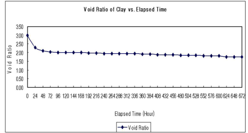
Figure 6. Decrease of void ratio.
