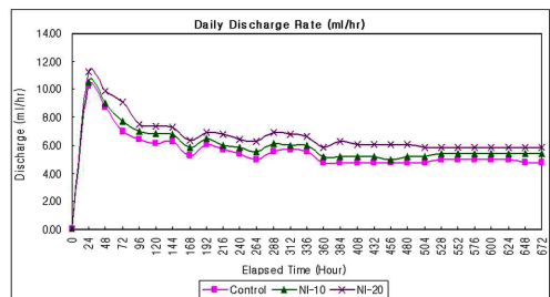
Figure 3. Discharge rate for time passing
