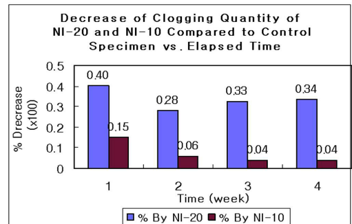
Figure 11. Clogging decrease after every week
