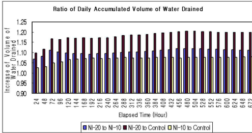
Figure 4. Ratio of daily accumulated volume of water drained
