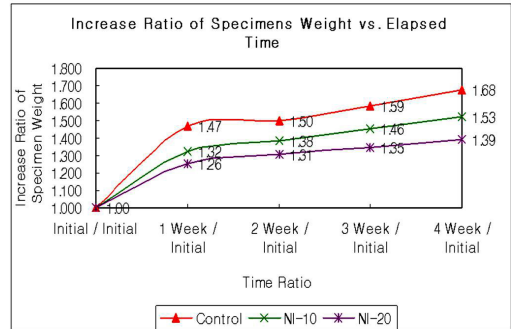
Figure 10. Increase ratio of specimen weights
