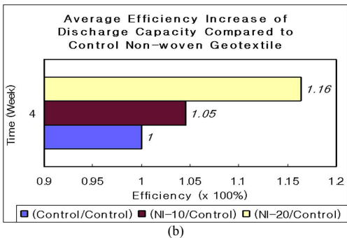
Figure 8. Increases of efficiency by using negative ion treated non-woven geotextiles in respect to volume of water drained (a) and discharge capacity (b)
