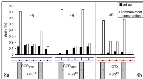
Figure 8. Geosynthetics strain
