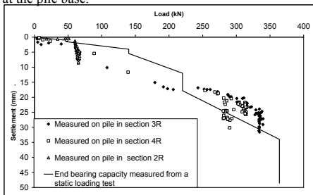
Figure 2. Comparison between the loads measured on pile head and the end bearing capacity of the static loading test
