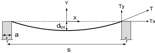
Figure 1: Parabolic approximation for reinforcement spanning adjacent columns
