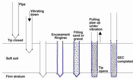
Figure 1 – Installation by the Displacement Method (Apud. Alexiew 2005)
