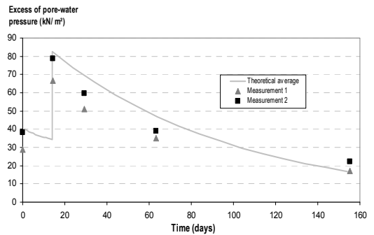
Figure 3 – Dissipation of the excess of pore-water pressures
