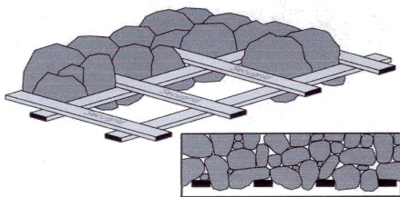
Figure 2. Interaction of aggregate with geogrid
