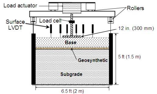
Figure 6. Schematic diagram of the pavement test facility
