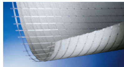
Figure 5. Combigrid® Geocomposite (geogrid reinforcement & needle punched nonwoven geotextile, firmly bonded between the cross laid reinforcement bars)
