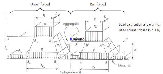
Figure 4. Increase of load distribution capacity with the use of geogrids (Giroud et al 1981)
