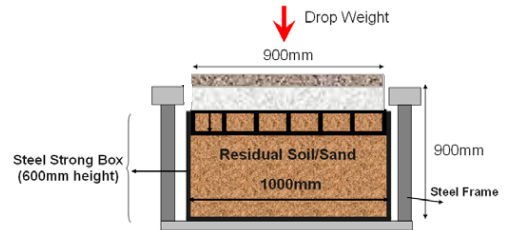
Figure 5. Setup of Test Configuration
