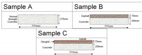
Figure 3: Sample Configuration for Impact Test
