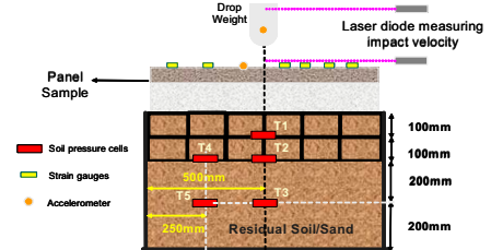
Figure 6. Instrumentation Set Up
