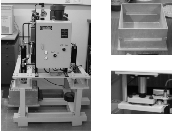
Figure 1 Equipment for DDI laboratory tests.
