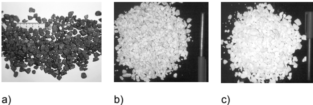
Figure 2 Granular materials used in the DDI laboratory tests: a) Aggregate 1, synthetic; b) Aggregate 2, granite; and c) Aggregate 3, limestone.
