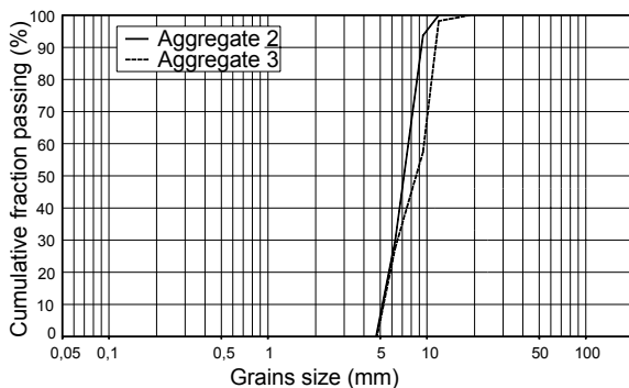
Figure 3 Particle size distributions, Aggregate 2 and Aggregate 3.
