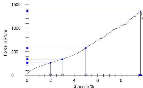
Figure 4. Tensile curve of the geogrid.
