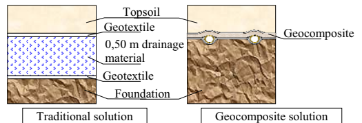
Figure 2. Drainage under embankment
