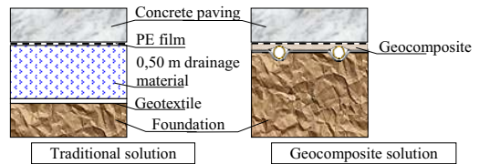
Figure 1. Drainage under pavement
