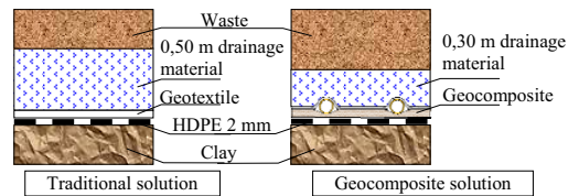
Figure 4. Drainage at bottom of landfill
