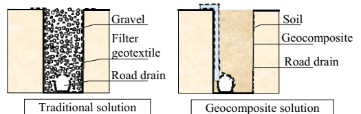
Figure 3. Drainage screen along roadside
