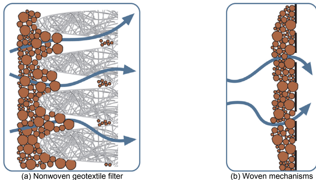
Figure 1. Diagrammatic presentation of main generic types of geotextiles
