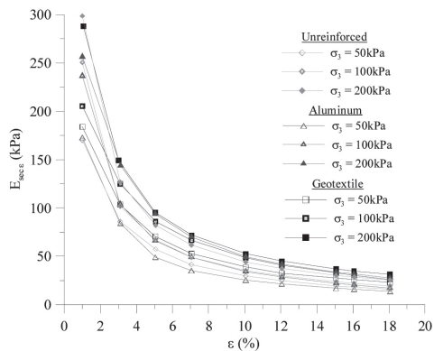
Figure 4. Stiffness versus strain curves from UU triaxial tests.
