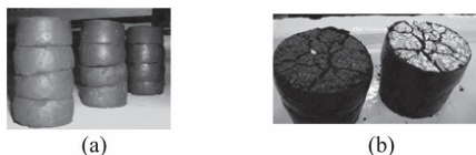
Figure 3. Specimens after failure. (a) Geotextile. (b) Aluminum.
