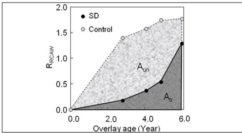
Figure 1. R_{RCAW} versus overlay age for an untreated and treated section.
