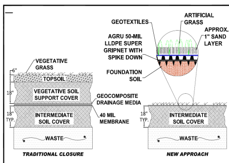
Figure 2 System Comparison
