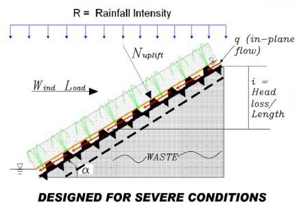
Figure 1. Forces and Flow Diagram
