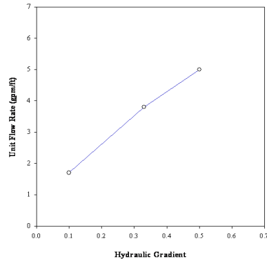
Figure 5 Flow Capacity
