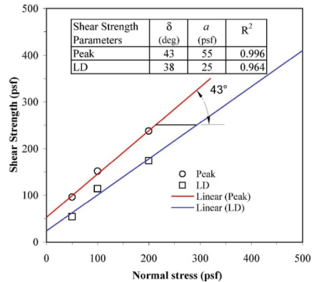
Figure 3 Interface Friction Results
