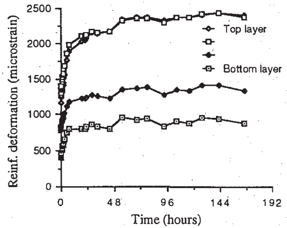
Fig. 4 - Reinforcement deformation vs time
