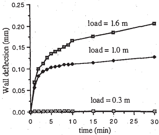
Fig. 2 - Wall deflection vs time (30 min. test)
