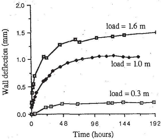
Fig. 3 - Wall deflection vs time
