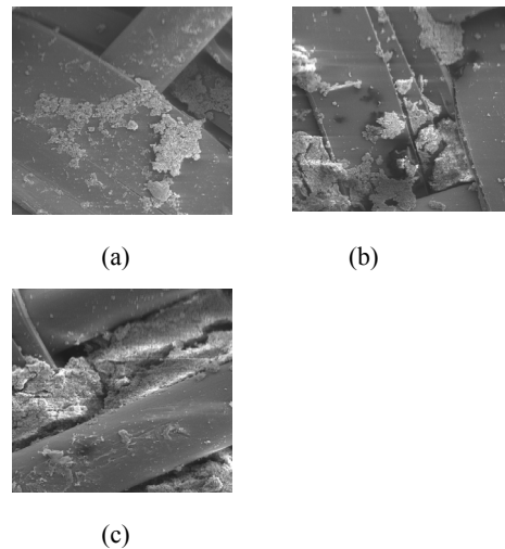
Figure 4-Woven geotextile clogging: (a) 30 days; (b) 60 days; (c) 90 days
