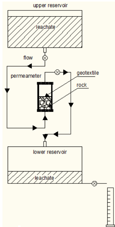
Figure.1 Layout of equipment used to measure permeability
