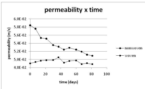
Figure.2 Variation of permeability x time
