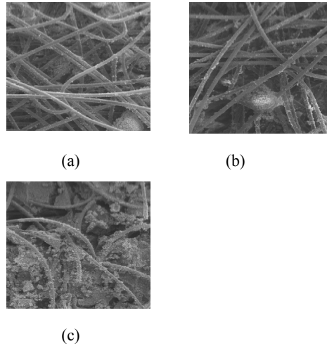
Figure 3-Nonwoven geotextile clogging: (a) 30 days; (b) 60 days; (c) 90 days
