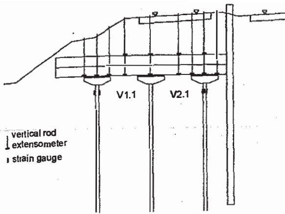
Fig. 3: Vertical rod extensometers
