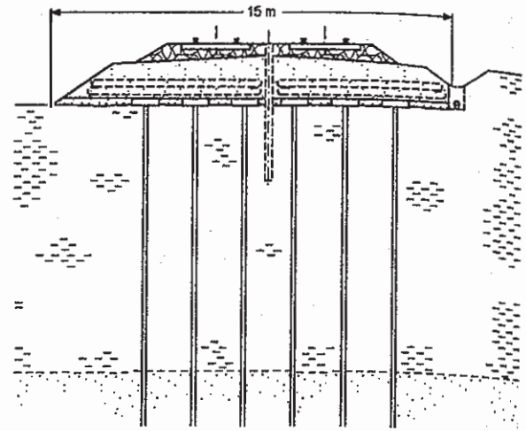
Fig. 1: Cross section of the embankment
