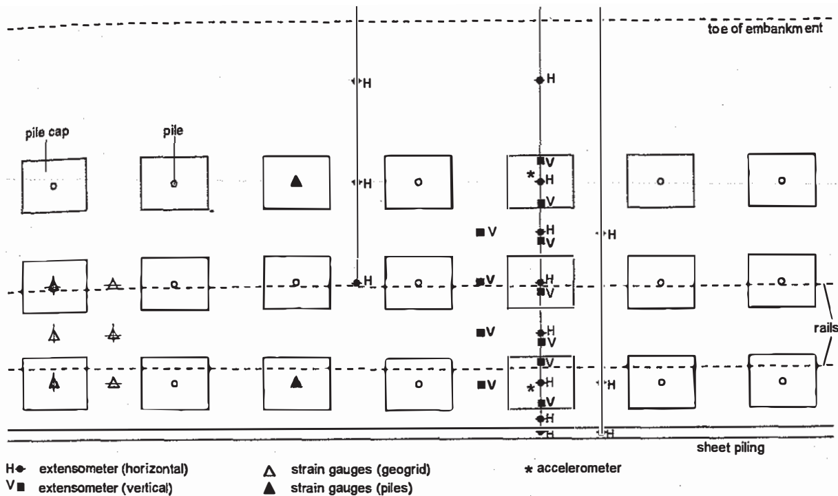
Fig. 2: Instrumentation of the monitoring section
