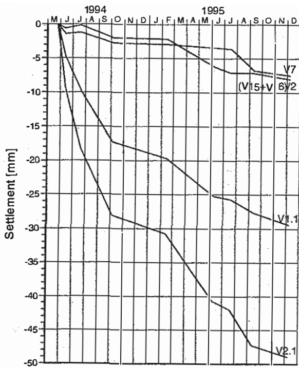
Fig. 5: Settlements with time
