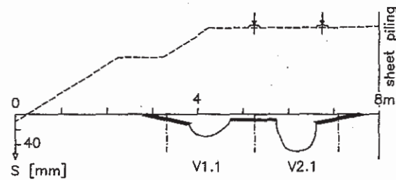
Fig. 4: Vertical displacements
