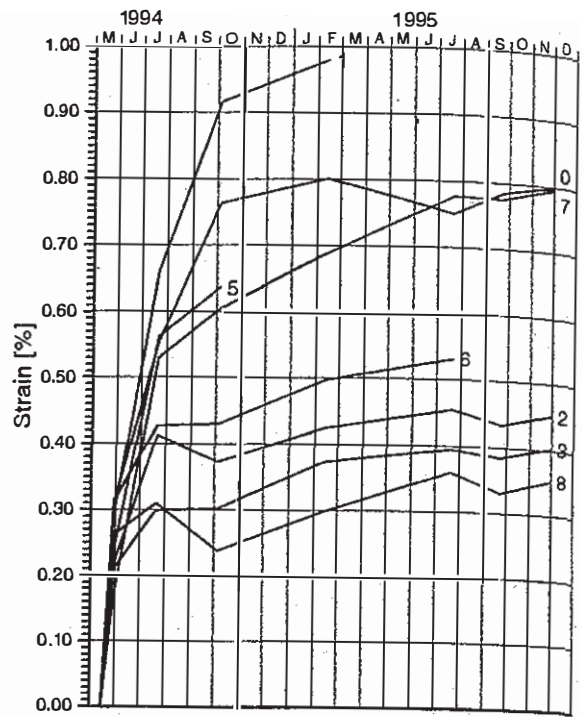
Fig. 6: Static geogrid strains with time
