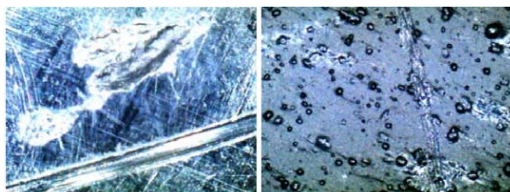
Figure 5. Scratching of the smooth and low asperity geomembrane after testing (50x).
