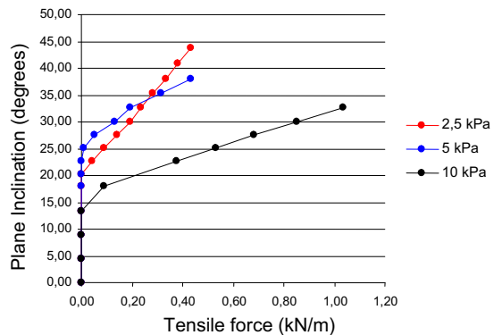
Figure 3. Typical test results for the ramp equipment with high-asperity GM sample.
