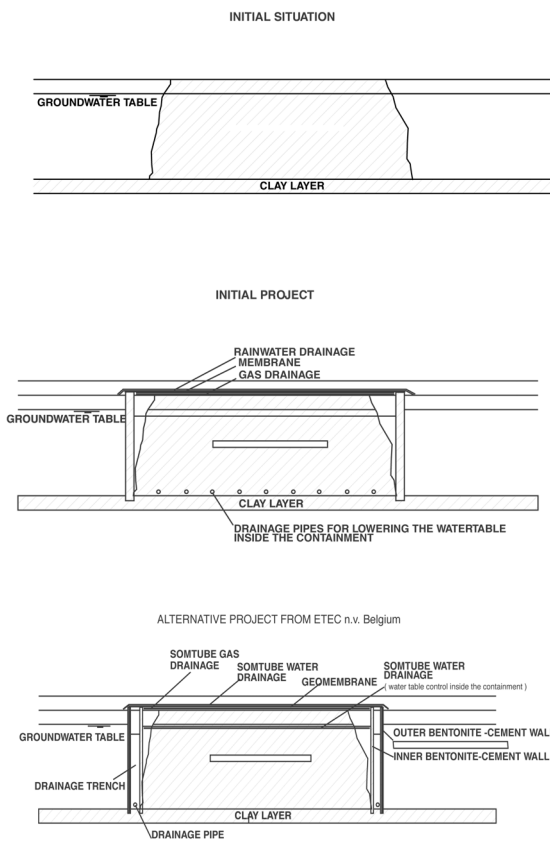
Figure 4. Containment Cross Sections
