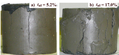
Figure 8. Specimens after tests (CTC)
