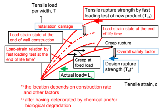
Fig. 1.7 Procedure to obtain the design rupture strength ( T_d ) of geosynthetic reinforcement under long-term static loading conditions compared with the value actually measured under ordinary non-critical condition ( L_a ).
