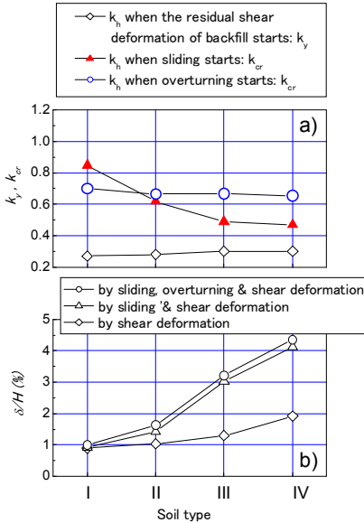
Fig. 1.6 a) Critical seismic coefficient when horizontal sliding or overturning failure starts ( k_{cr} ) and assumed yield k_h value above which residual deformation of reinforced backfill takes place ( k_y ); and b) calculated residual horizontal displacements at the crest of the wall for different soil types (Horie et al., 1998).
