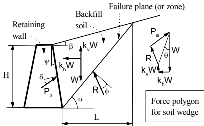
Fig. 1.3 Retaining wall with unreinforced backfill having a single linear failure plane under general seismic loading conditions (Koseki et al., 1997).
