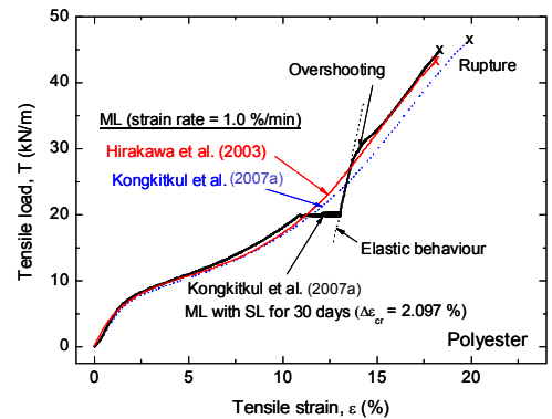
Fig. 1.9 Comparison of tensile load - strain relations from three ML tests with and without creep loading for 30 days at an intermediate load level, a PET geogrid (Kongkitkul et al., 2007a).
