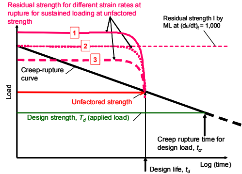
Fig.1.8 Effects of strain rate at rupture on residual strength (Tatsuoka et al., 2004)
