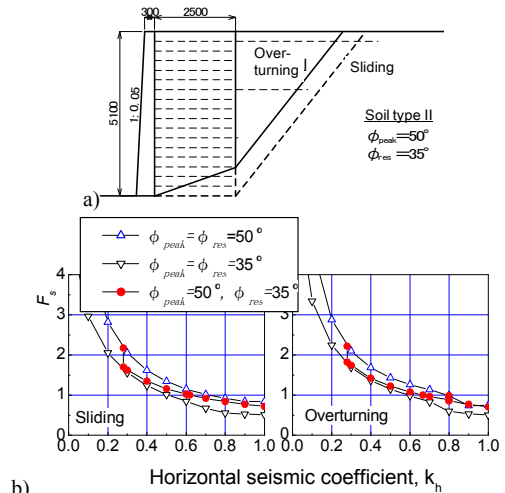
Fig. 1.5 a) Typical configurations of GRS RW with FHR facing and critical failure planes (unit in mm); and b) results of stability analysis for soil type II (Table 1.3) (Horii et al., 1998).
