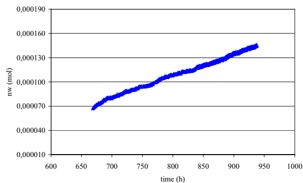
Figure 4. Water vapour (wv) permeated through the specimen after the steady-state achievement.
