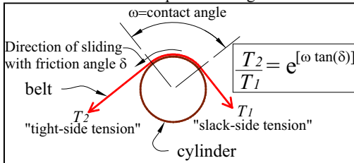
Figure 2. Schematic of Euler-Eytelwein belt-friction model.
