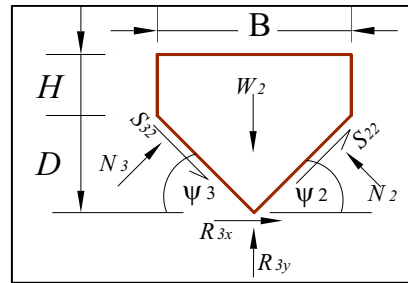
Figure 5. Free-body diagram of soil block 2.
