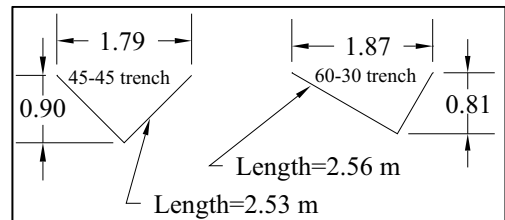
Figure 6. Comparison of two V-trench geometries that provide equal pullout resistance.
