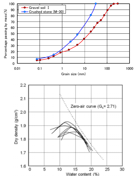
Fig. 6. a) Grading curves; and b) compaction curves (modified Proctor) of the main backfill
