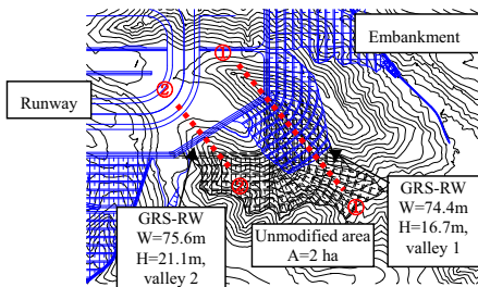
Fig. 3. Plan view of the eastern end of the runway (①-① and ②-② indicate cross-sections shown in Fig. 4)
