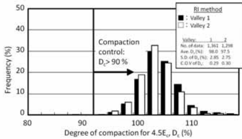
Fig. 8. Histogram of degree of compaction D_c
