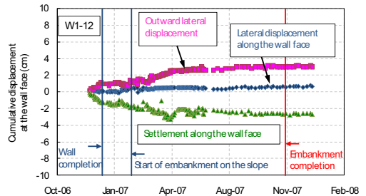
Fig.10. Displacements at the wall face, 13 th geogrid layer in the GRS wall in valley 1.
