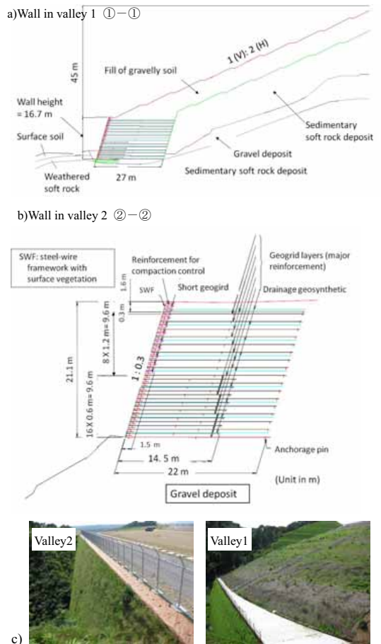
Fig. 4. Cross-sections of the two GRS-RW
