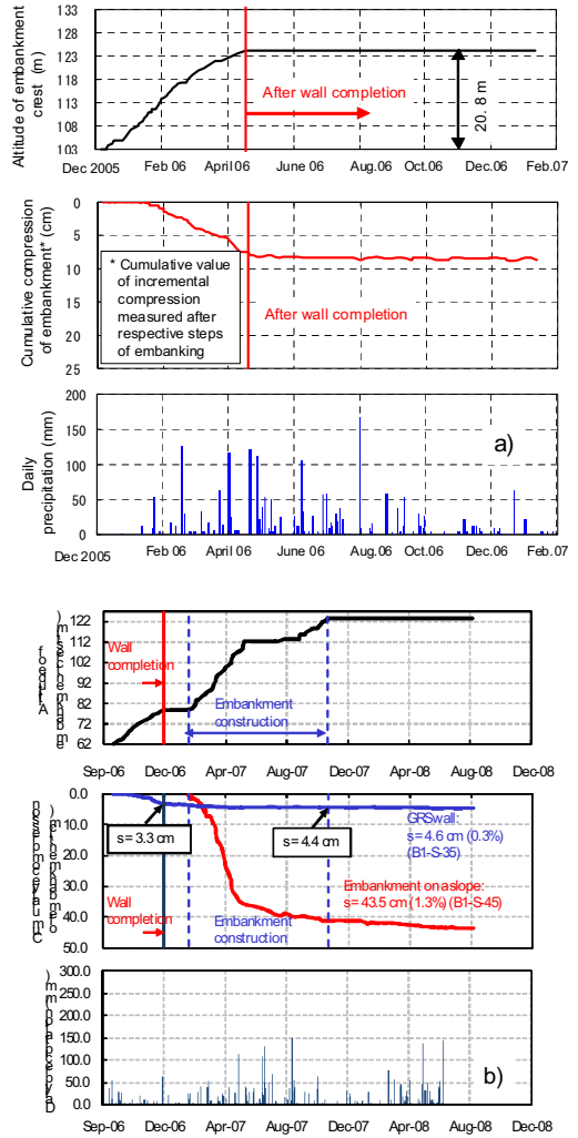
Fig. 9 a) Deformation of the wall and embankment on a slope, valley 1; and b) deformation of the wall, valley 2
