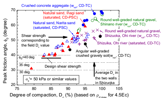
Fig. 12. Summary of \phi_0 - D_c (for 4.5E_c ) relations from drained TC and PSC tests at confining pressures of around 20 - 50 kPa. Note: w_{opt} in the parenthesis indicates that, when tested, the specimens were moist; and the others were saturated (Kiyota et al., 2009).
