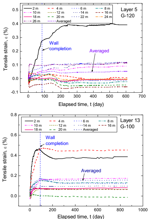
Fig. 11. Tensile strains in representative geogrid layers
