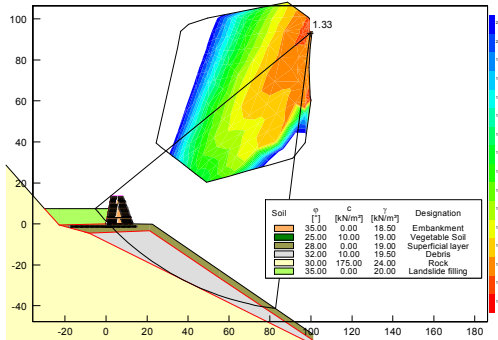
Figure 6. Example of overall stability calculation
