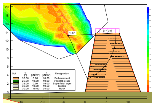
Figure 5. Example of internal stability calculation (back side)
