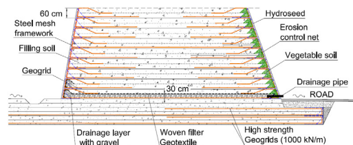
Figure 4. Section detail. Drainage layer with a woven filter
