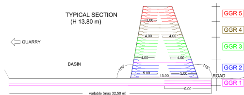
Figure 3. Structural configuration of the embankment
