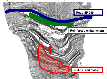
Figure 2. plan of the quarry, sliding body, reinforced embankment and road at the toe.
