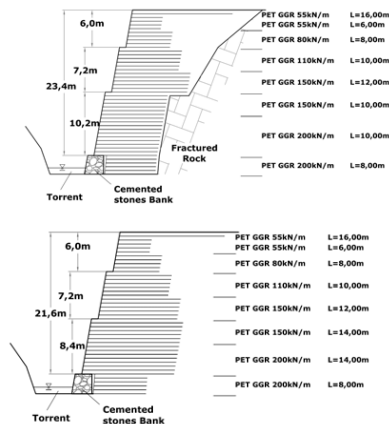
Figure 2. Cross sections of the two situations of the reinforced steep slope
