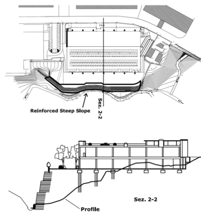
Figure 1. Plan view and typical cross section of the reinforced steep slope
