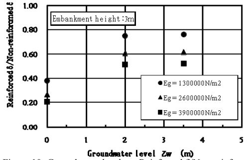
Figure 10. Groundwater level vs. Reinforced \delta /Non-reinforced \delta ( H=3\text{ m} )
