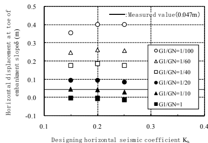
Figure 7. Relationship between the design horizontal seismic coefficient and toe-of-slope horizontal displacement
