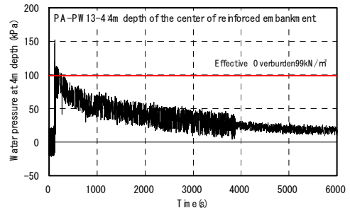
Figure 3. Pore water pressure in the soil
