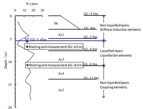
Figure 4. SPT N-value and geological profile
