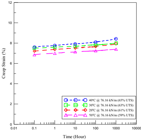
Figure 5 Long term creep curves for 76.16 kN/m tensile load at 10°C, 20°C, 30°C, and 40°C.
