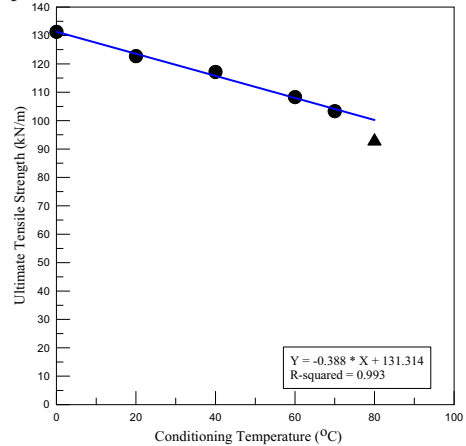
Figure 4 Average tensile strength versus temperature for the test geogrid.
