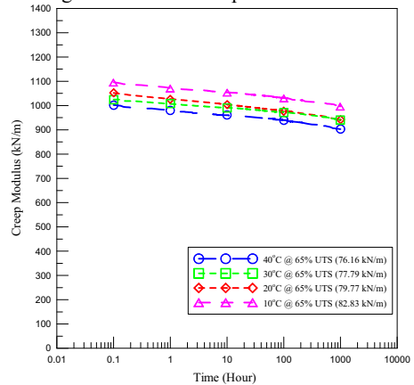
Figure 8 Creep modulus curves under 65% UTS loading at various test temperatures.
