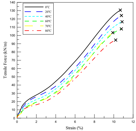
Figure 3 Typical wide width tensile test results of longitudinal ribs of the test geogrid at various temperatures.
