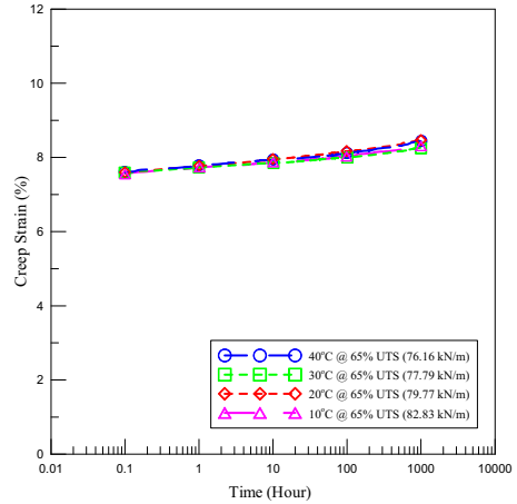
Figure 7 Long term creep curves under 65% UTS loading at various test temperatures.
