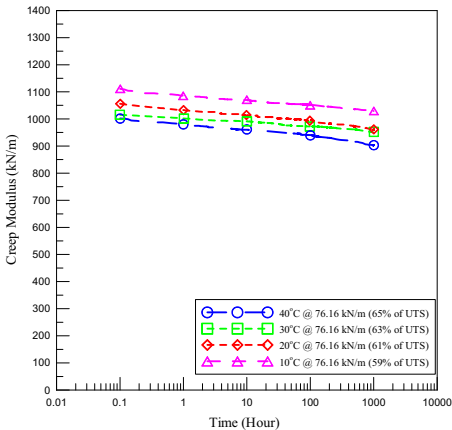
Figure 6 Creep modulus versus time curves for 76.16kN/m tensile load at 10°C, 20°C, 30°C, and 40°C.
