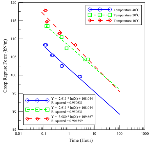
Figure 9 Creep rupture data and regression lines at various test temperatures.
