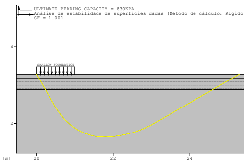
Figure 7. Safety factor value about 1 obtained with reinforcement to ultimate bearing capacity equal 830kPa.
