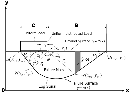
Figure 3. Geometric quantities defining the shape of the shear surface in a homogenous bearing media, Hopkins et al. (2005).
