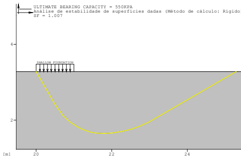
Figure 6. Safety factor value about 1 obtained without reinforcement to ultimate bearing capacity equal 550kPa.
